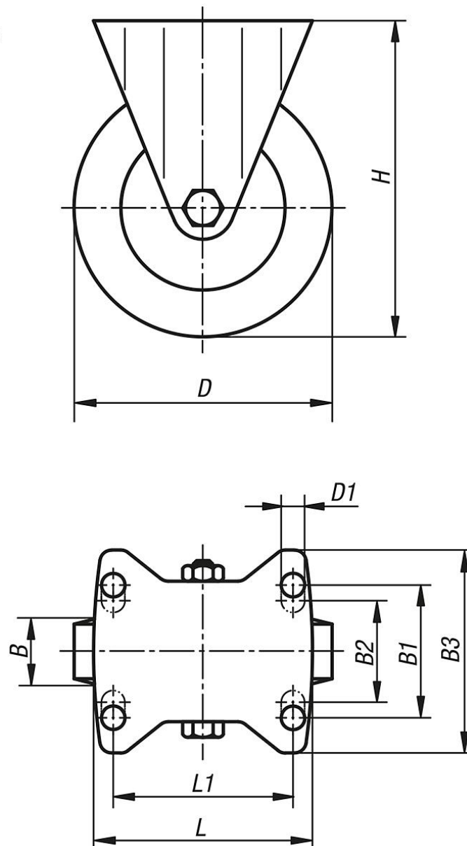
Bockrolle
